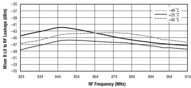
Figure 31. Mixer B LO to RF Leakage vs Frequency and Temperature
