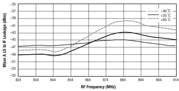
Figure 29. Mixer A LO to IF Leakage vs Frequency and Temperature
