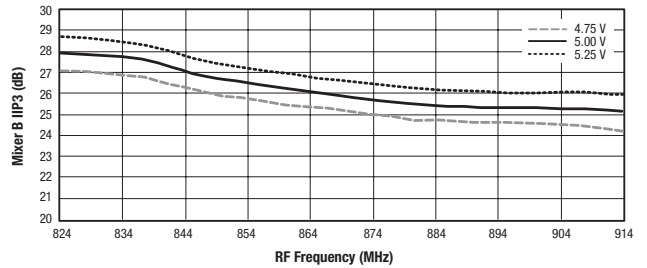
Figure 16. Mixer B IIP3 vs Frequency and Supply Voltage
