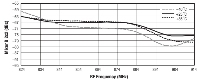
Figure 26. Mixer B 2RF-2LO vs Frequency and Temperature
