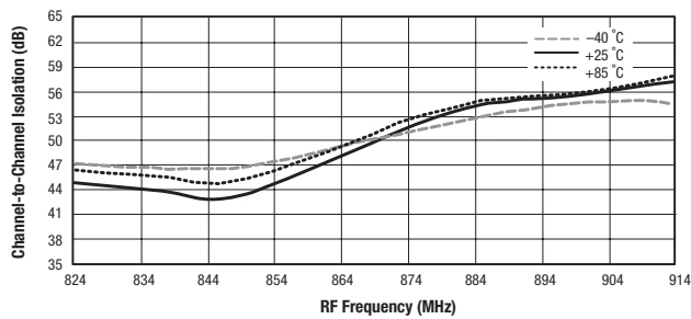
Figure 33. Channel A to Channel B IF Isolation vs Frequency and Supply Voltage
