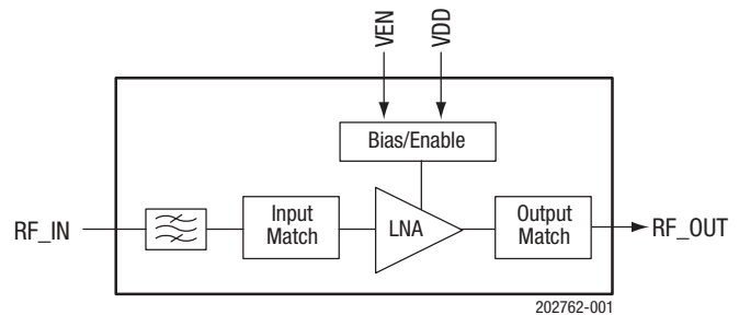
Figure 1. SKY65709-51 Block Diagram
